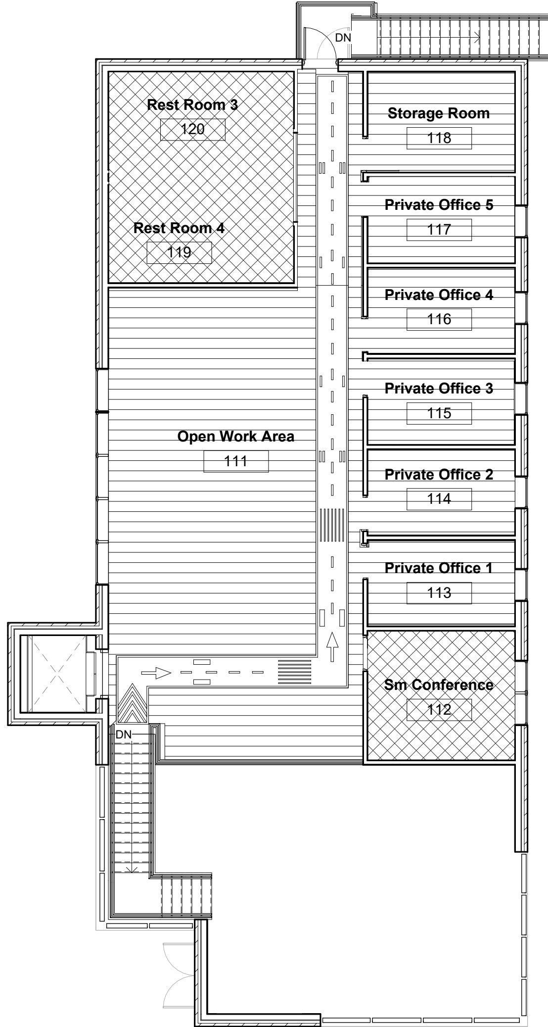
② LEVEL 2 FLOOR FINISH PRESENTATION 1/8" = 1'-0"
