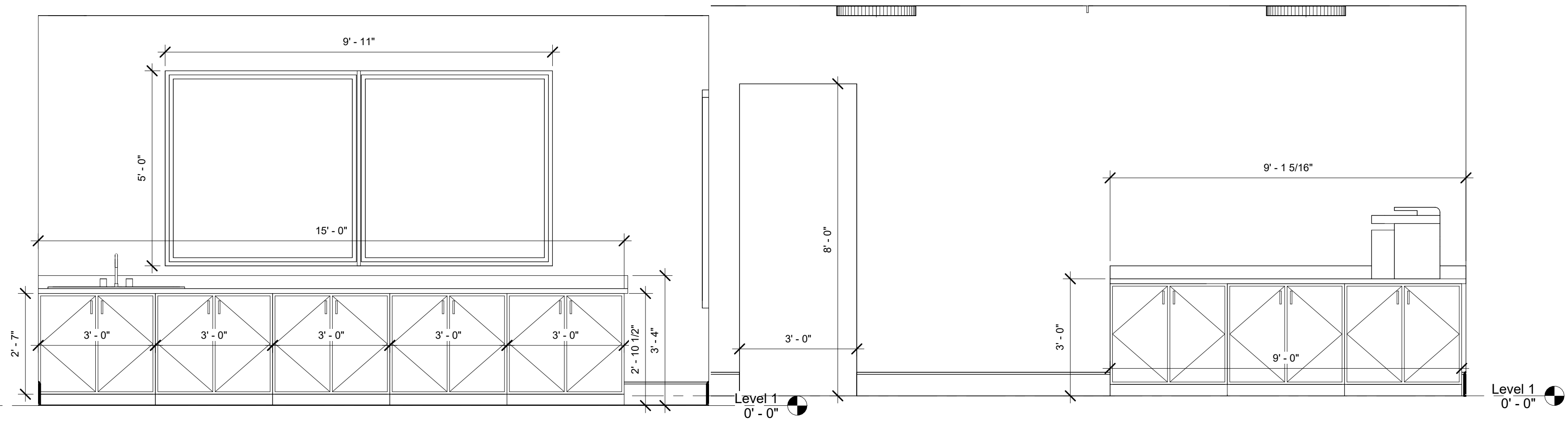
③ RECEPTION STORAGE AREA IN COAT ROOM 1/2" = 1'-0"
