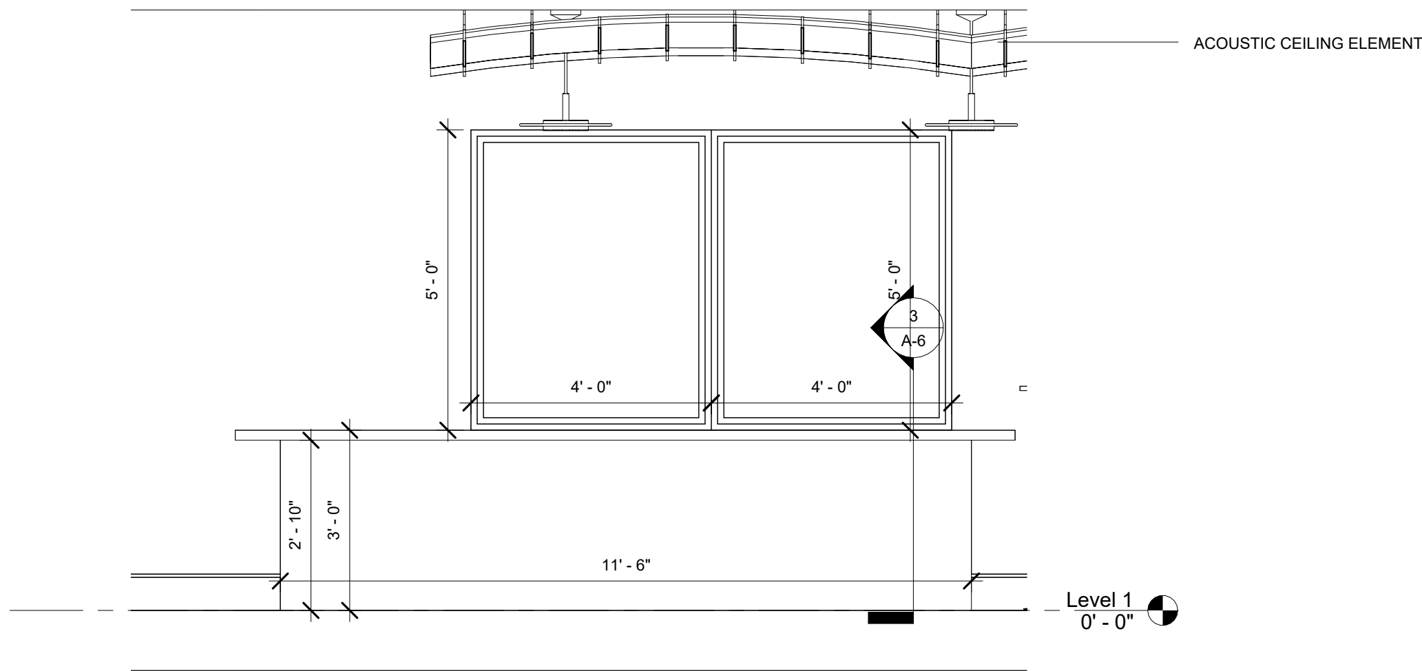
1 CAFE ELEVATION 1/2" = 1'-0"
