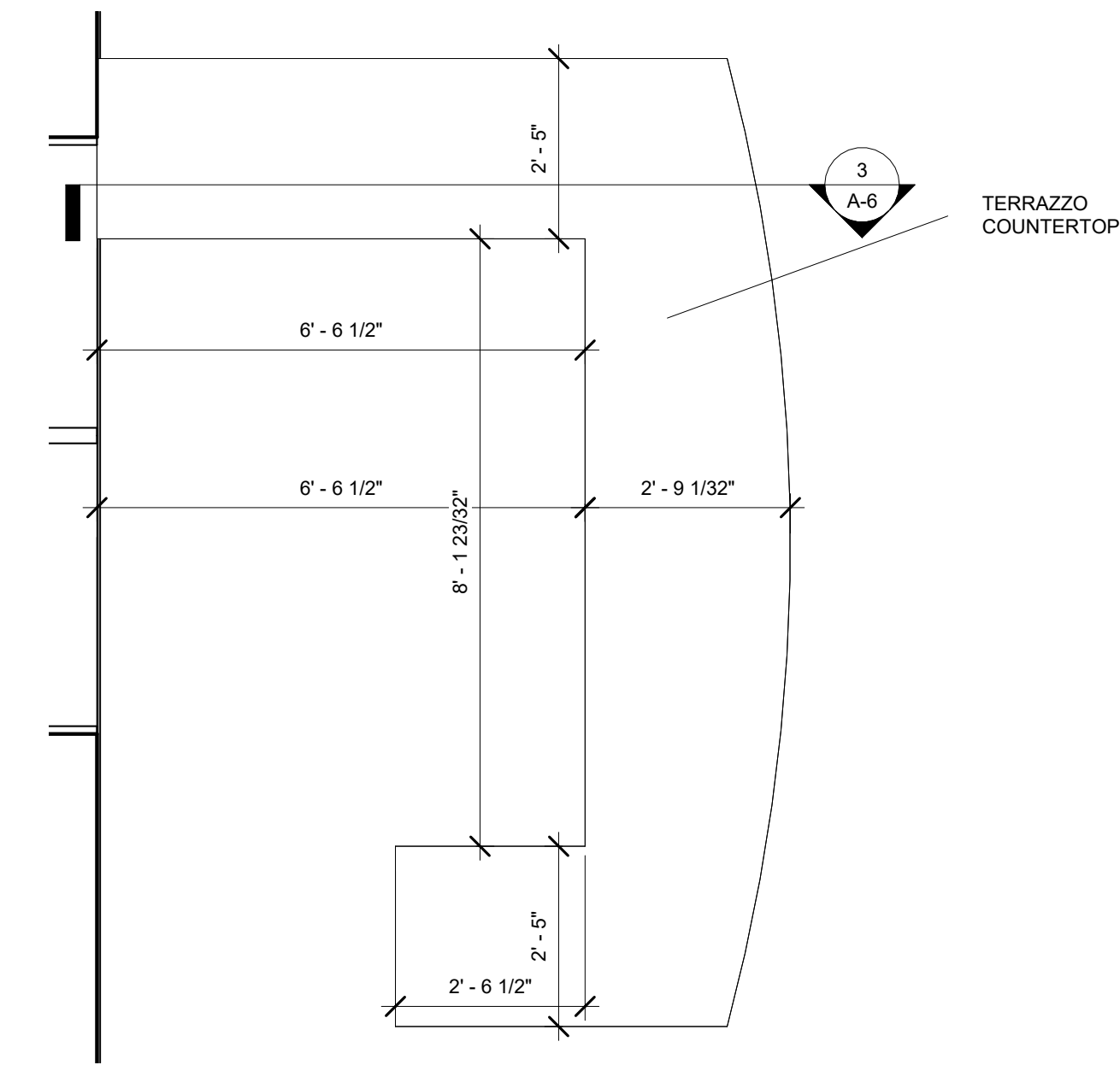
2 CALLOUT 1 CAFE 1/2" = 1'-0"
