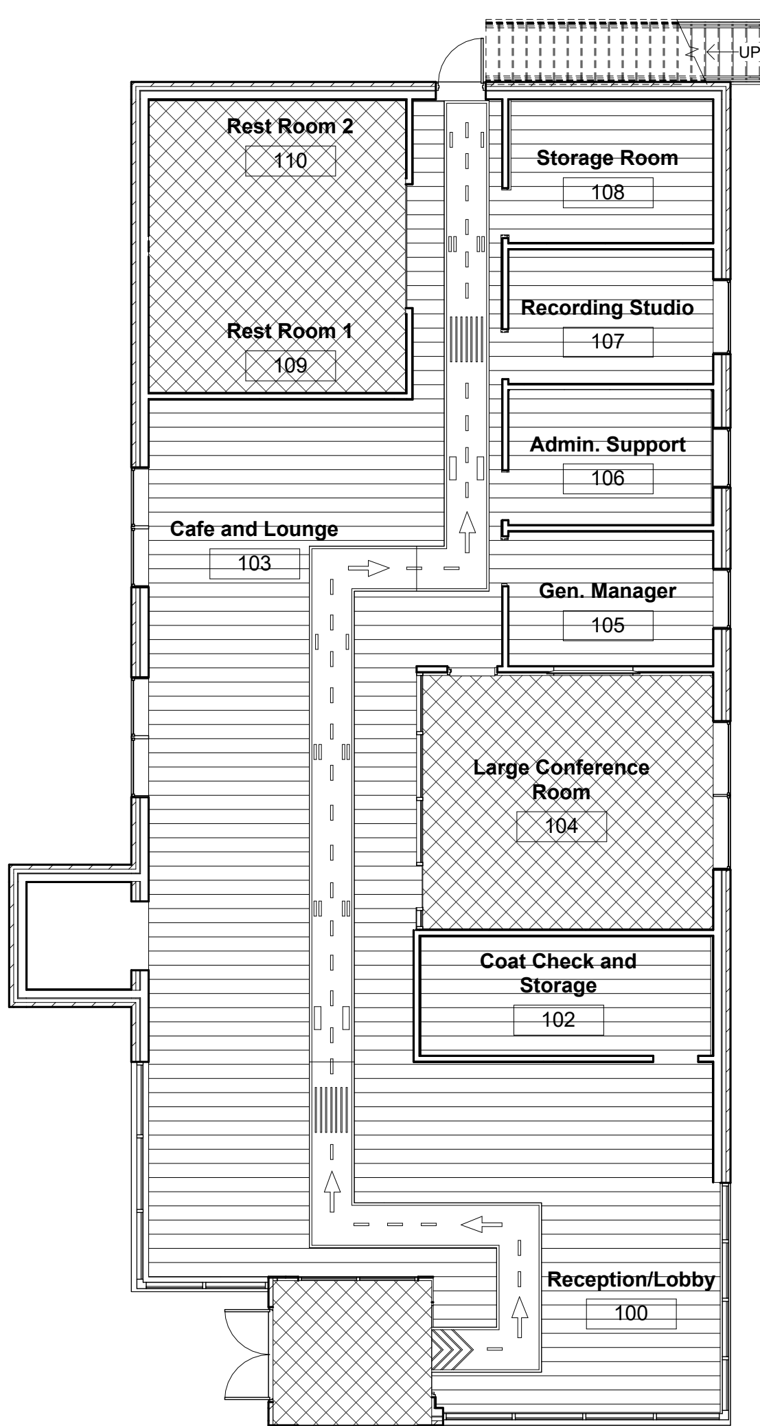
① LEVEL 1 FLOOR FINISH PRESENTATION 1/8" = 1'-0"
