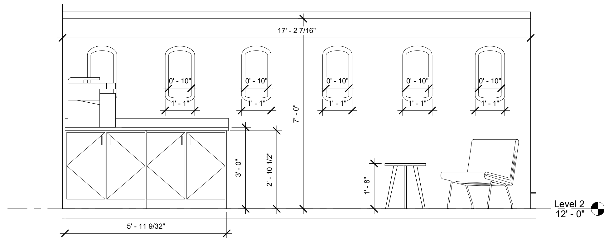
② PRINTING AREA ELEVATION 1/2" = 1'-0"
