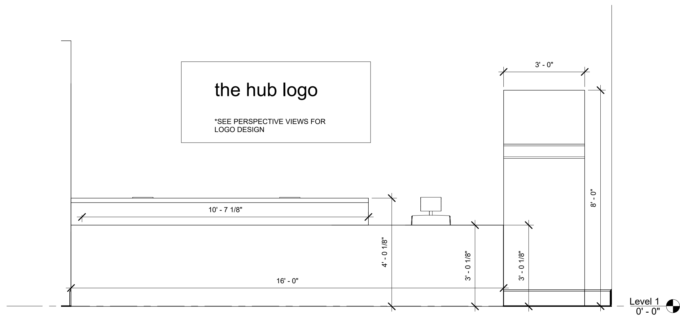
② RECEPTION DESK ELEVATION 1/2" = 1'-0"
