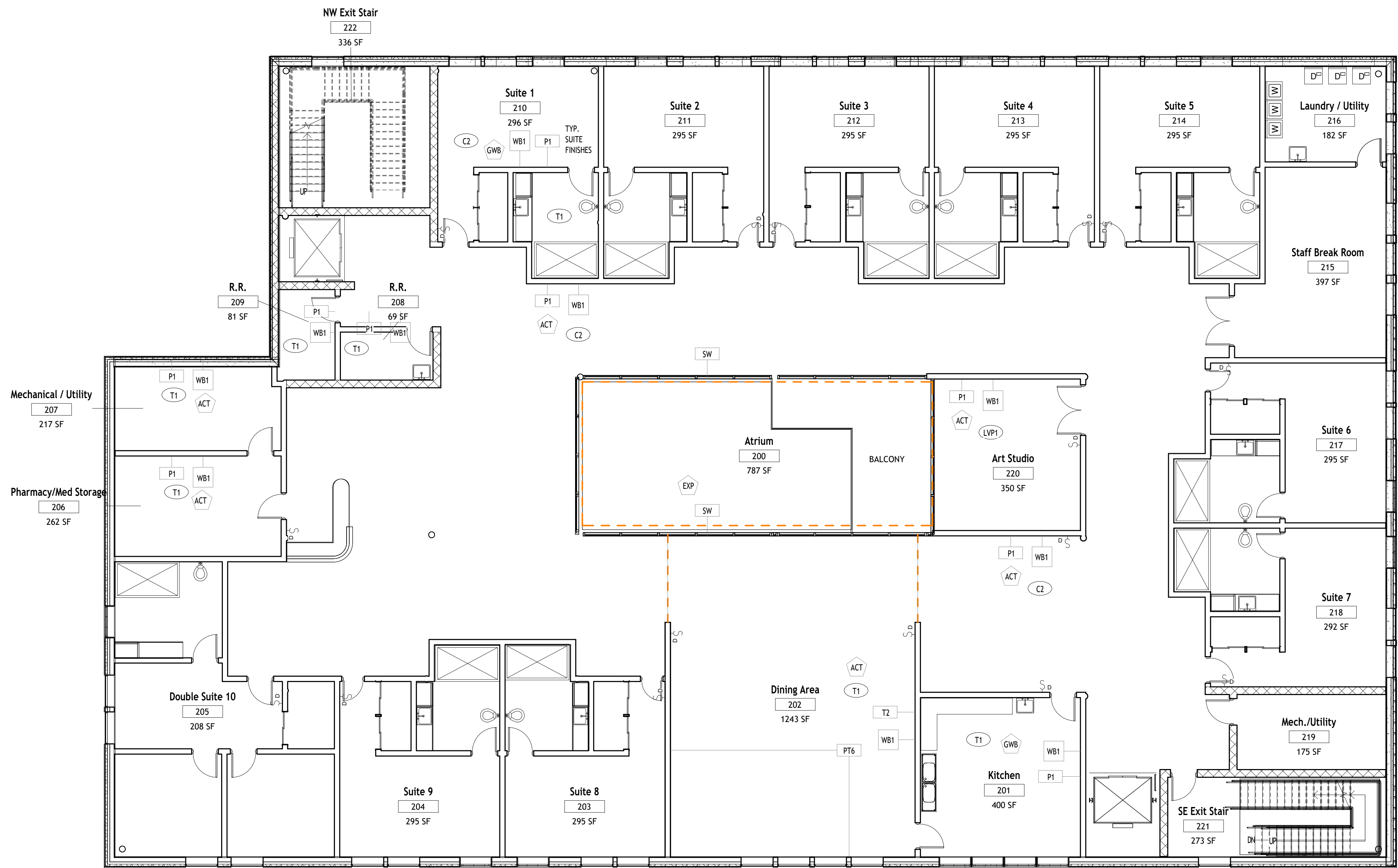
1 Second Floor Architectural Plan 1/8" = 1'-0"
