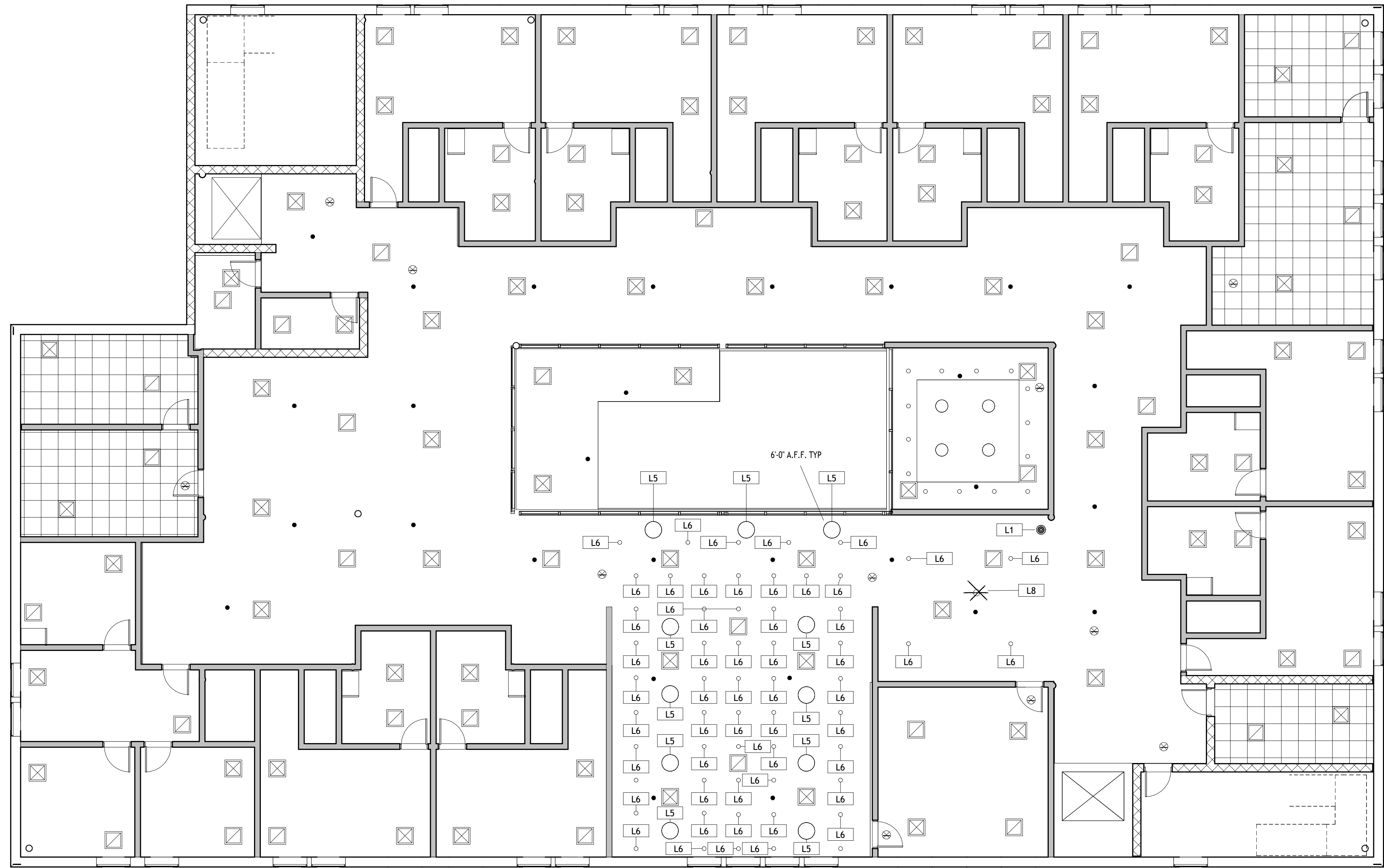
① Second Floor Architectural Ceiling Plan 1/8" = 1'-0"
