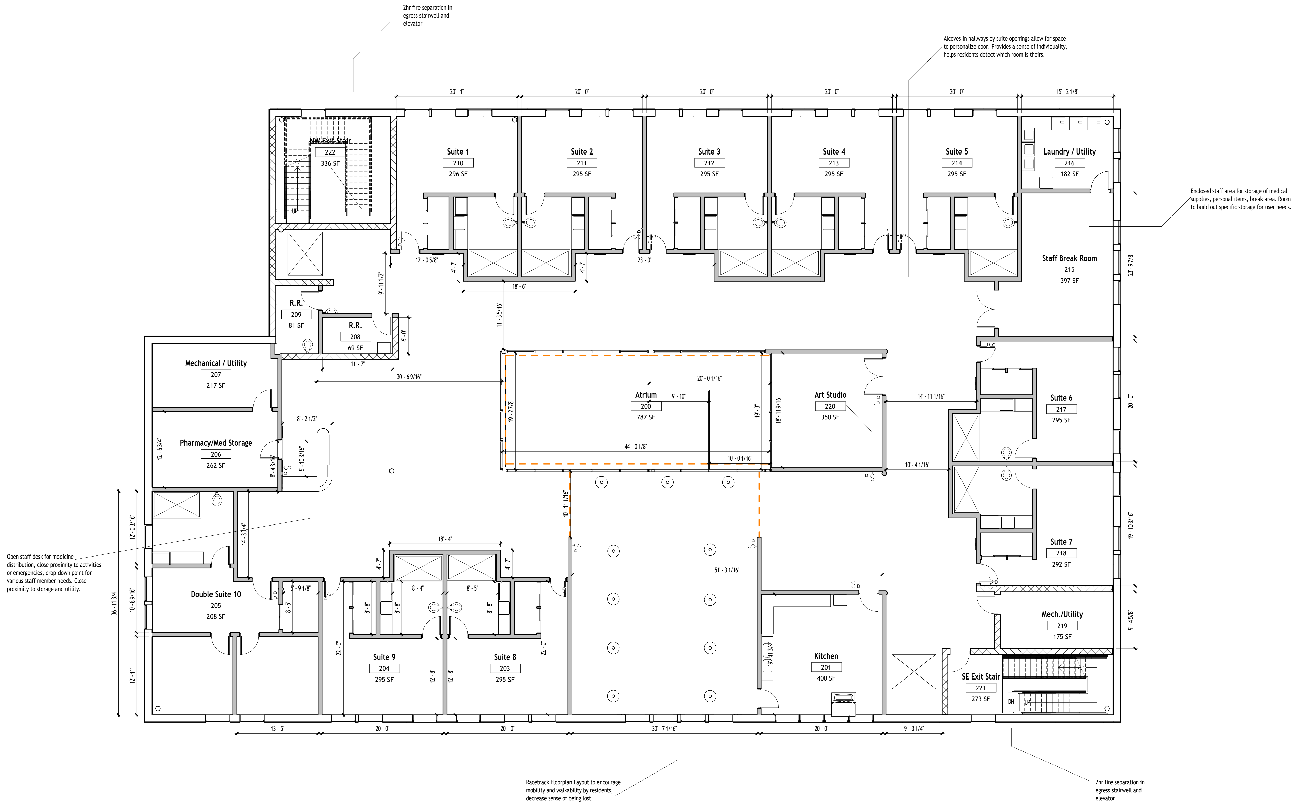
① Second Floor Architectural Plan 1/8" = 1'-0"
